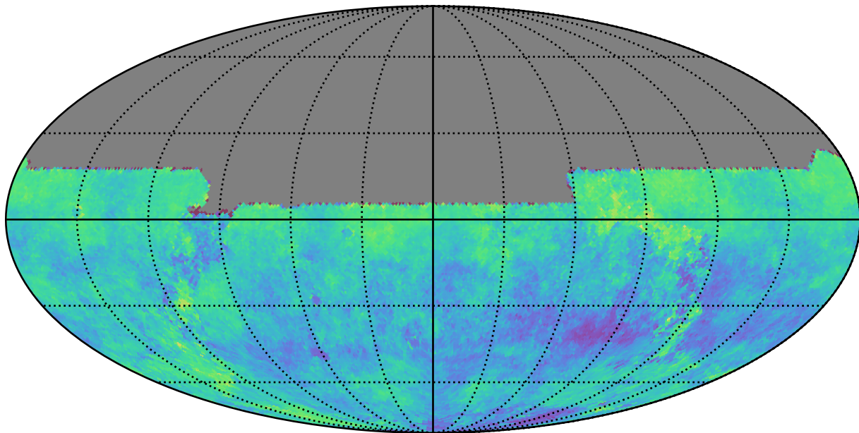
too_5_4v3.4_10yrs u: Kuiper rotSkyPos
