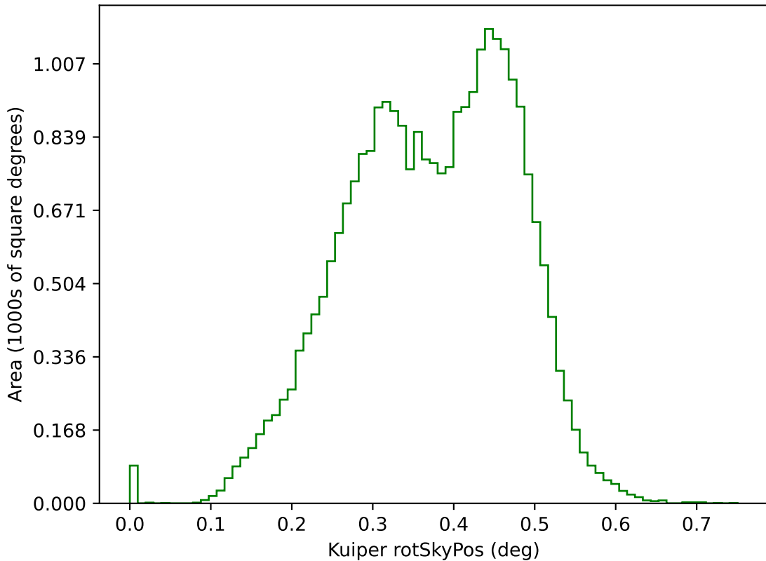
too_5_4v3.4_10yrs g: Kuiper rotSkyPos
