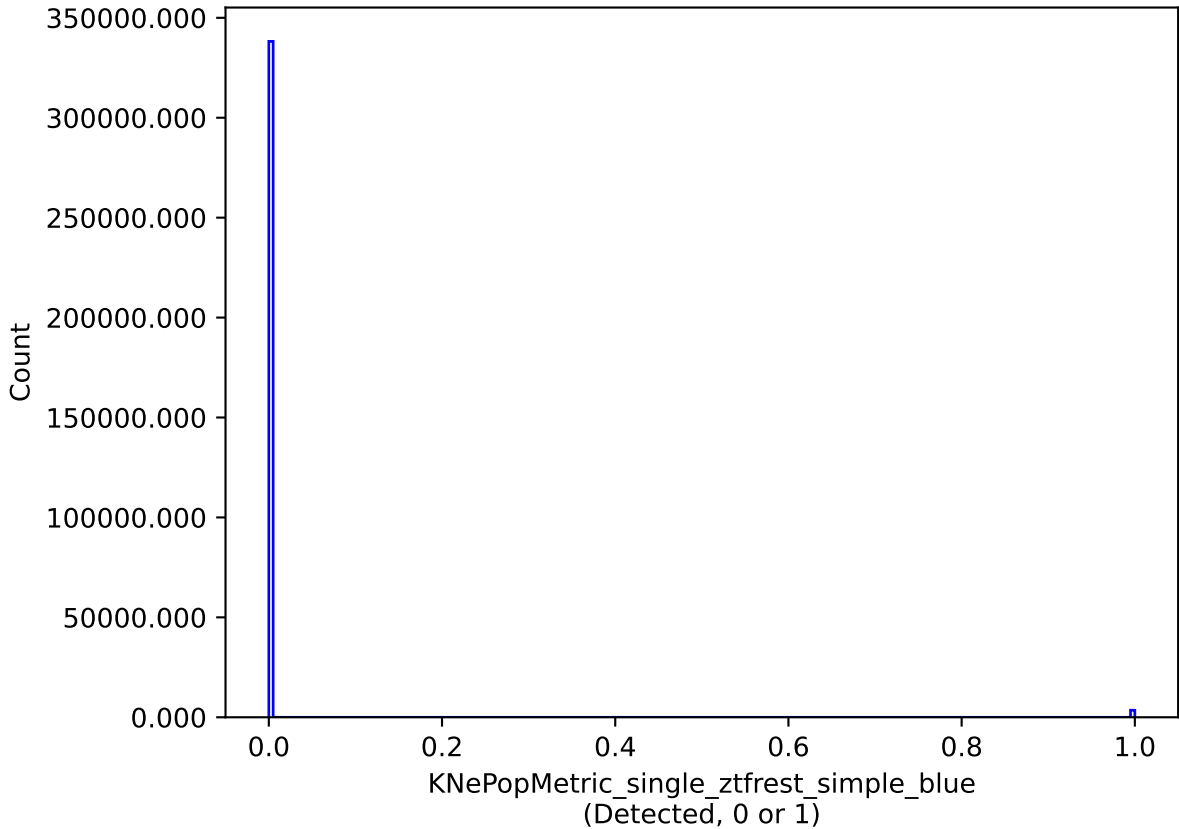
too_5_4v3.4_10yrs single model: KNePopMetric_single_ztfrest_simple_blue
