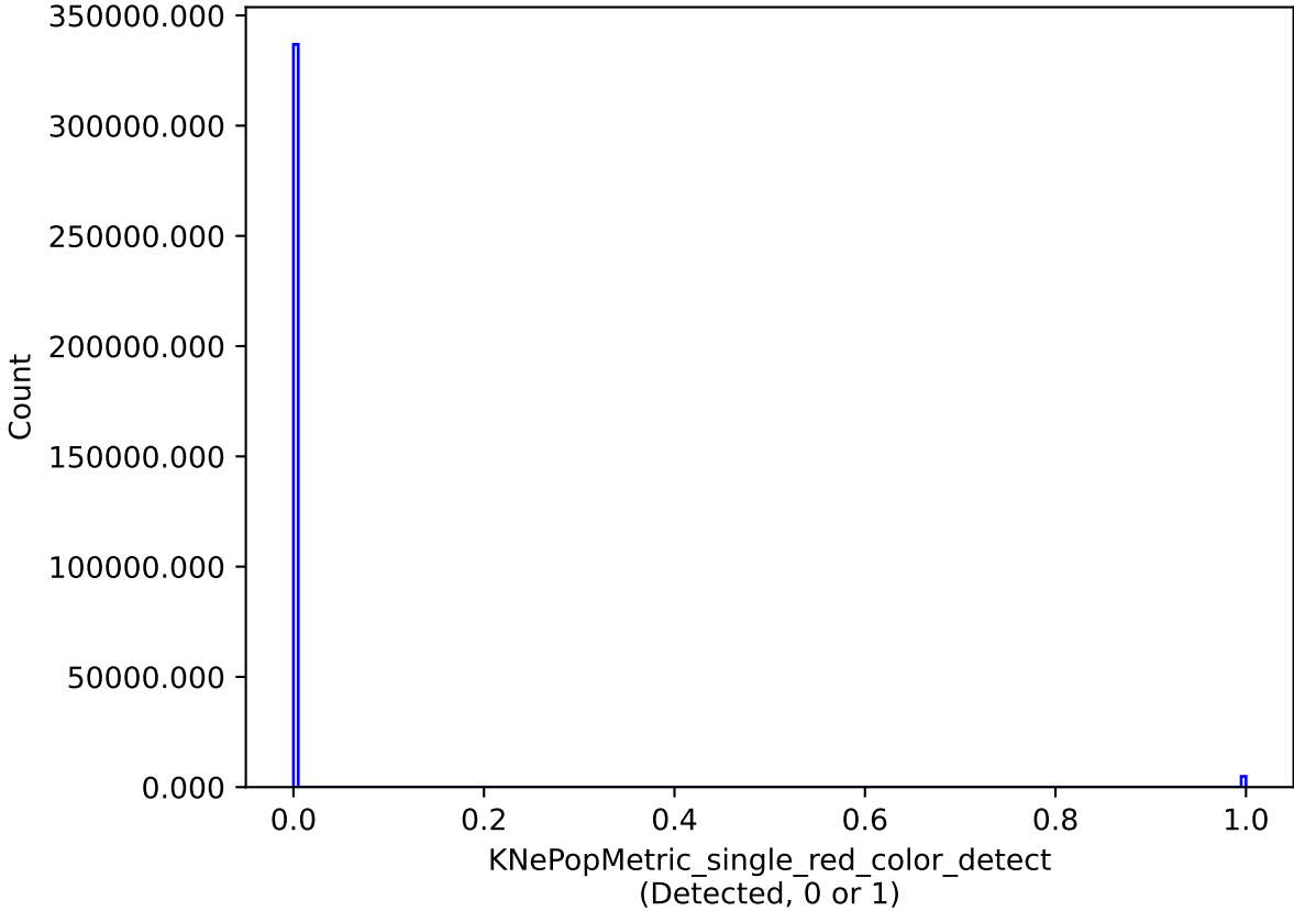
too_5_4v3.4_10yrs single model: KNePopMetric_single_red_color_detect
