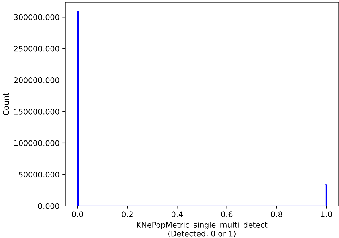
too_5_4v3.4_10yrs single model: KNePopMetric_single_multi_detect
