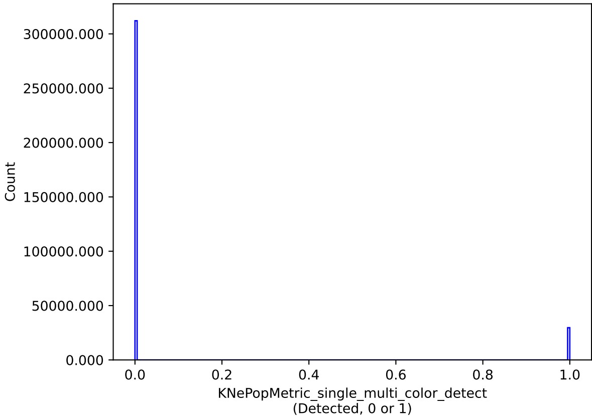
too_5_4v3.4_10yrs single model: KNePopMetric_single_multi_color_detect
