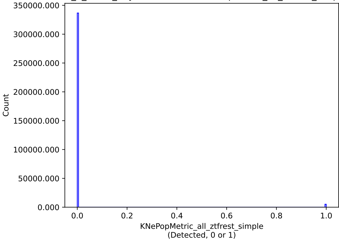
too_5_4v3.4_10yrs all models: KNePopMetric_all_ztfrest_simple
