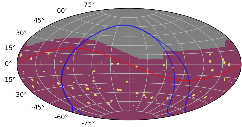
too_5_4v3.4_10yrs all models: KNePopMetric_all_red_color_detect
