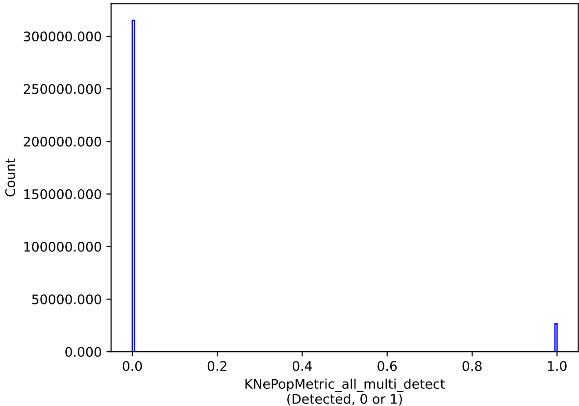
too_5_4v3.4_10yrs all models: KNePopMetric_all_multi_detect
