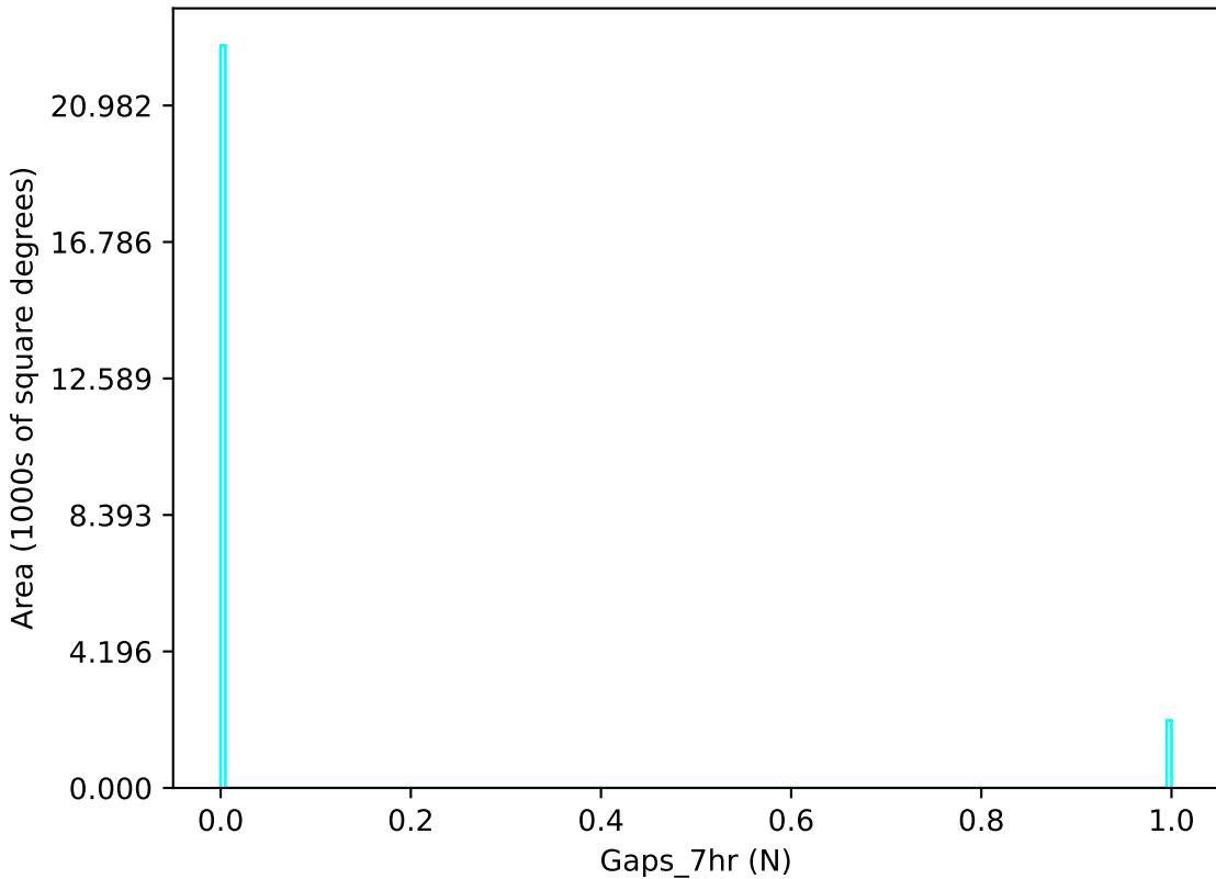
too_5_4v3.4_10yrs u band: Gaps_7hr
