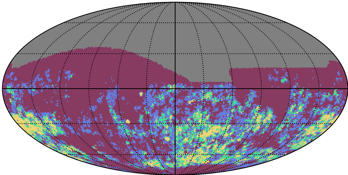
too_5_4v3.4_10yrs i band: Gaps_7hr
