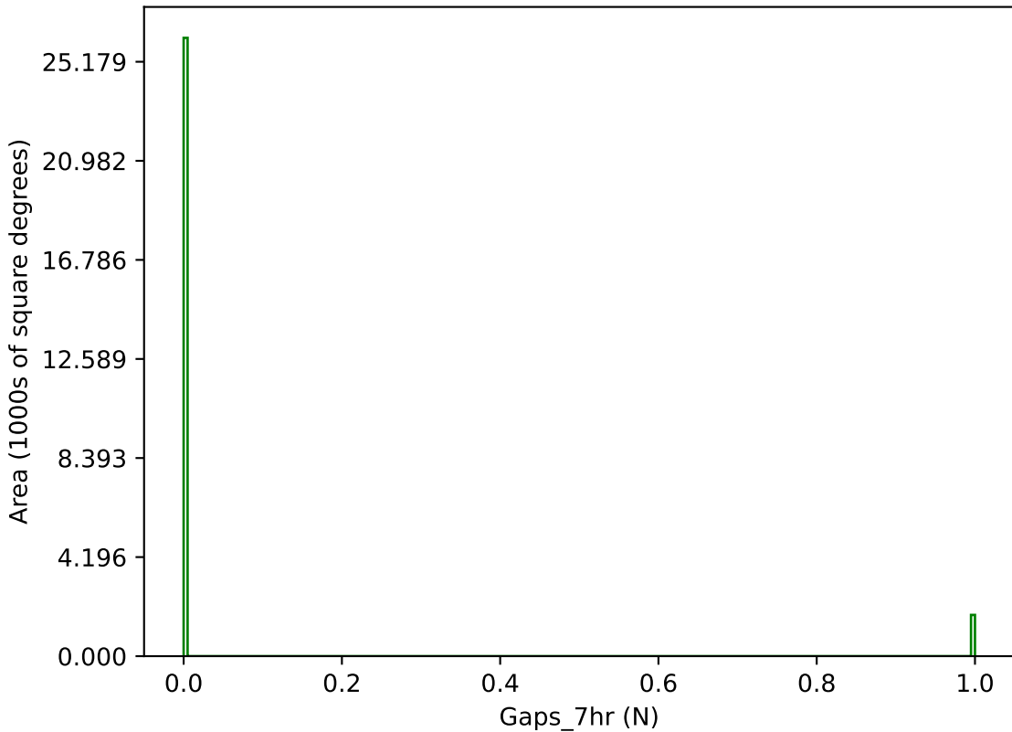
too_5_4v3.4_10yrs g band: Gaps_7hr
