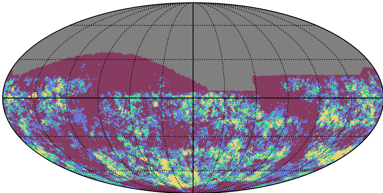
too_5_4v3.4_10yrs z band: Gaps_3hr
