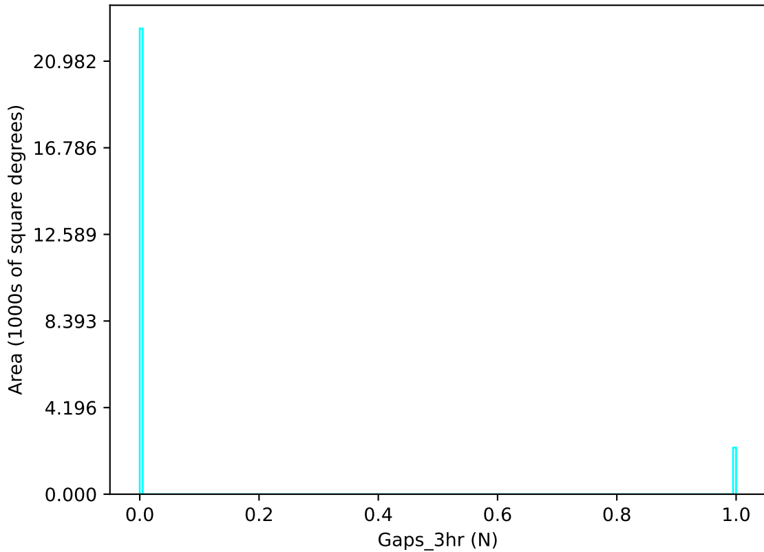
too_5_4v3.4_10yrs u band: Gaps_3hr
