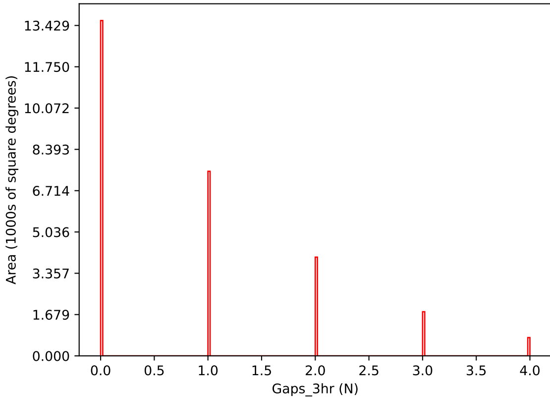
too_5_4v3.4_10yrs i band: Gaps_3hr
