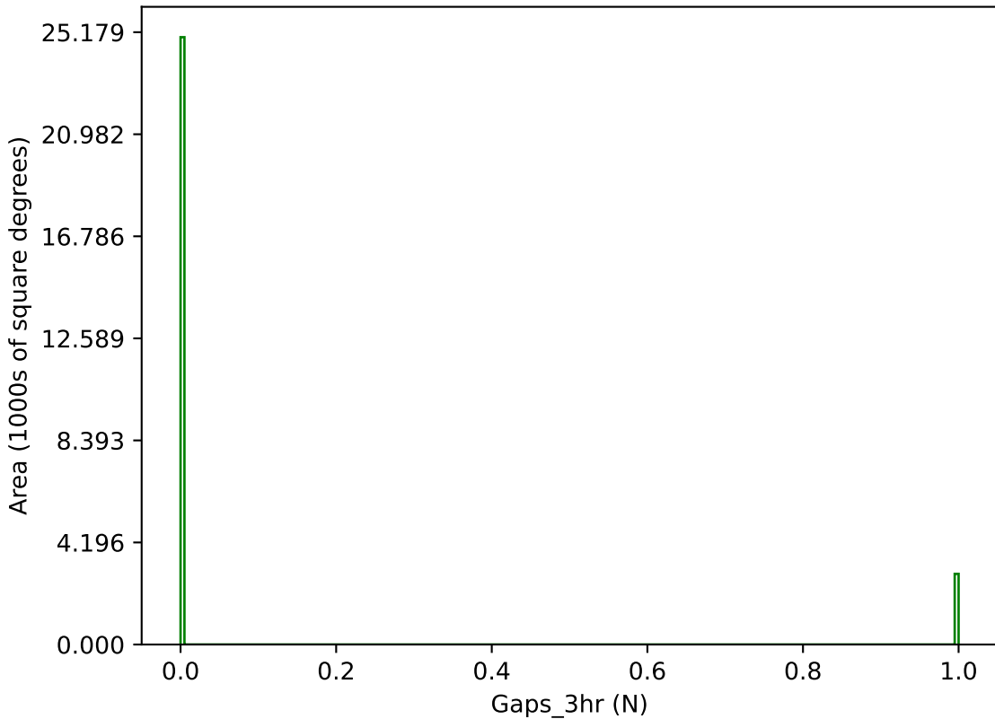
too_5_4v3.4_10yrs g band: Gaps_3hr
