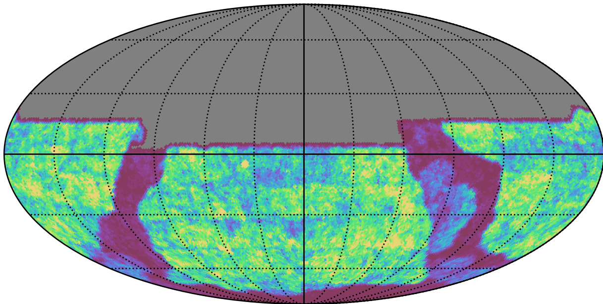
too_5_4v3.4_10yrs y band: Gaps_24hr
