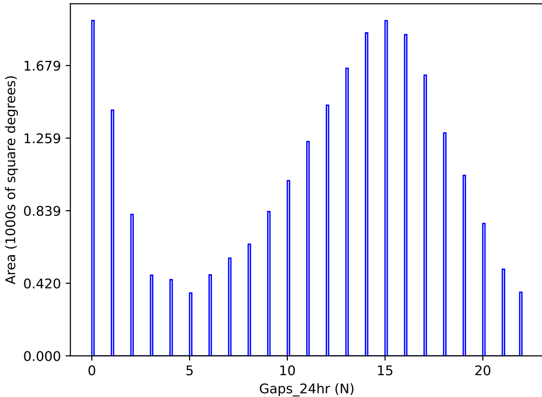
too_5_4v3.4_10yrs y band: Gaps_24hr
