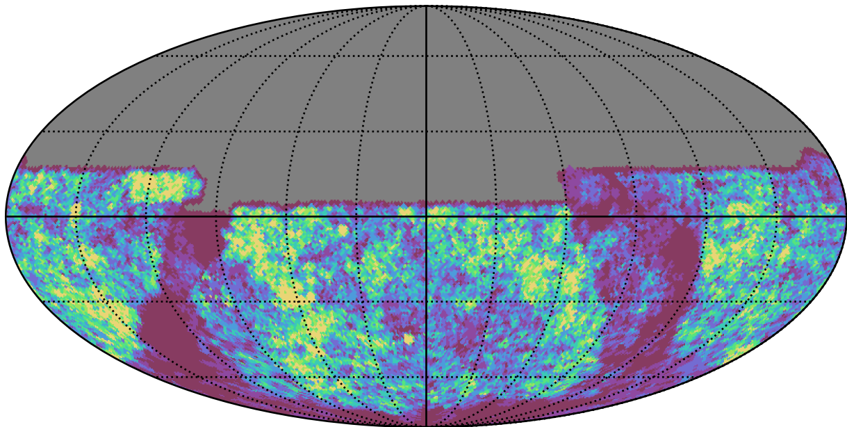
too_5_4v3.4_10yrs u band: Gaps_24hr
