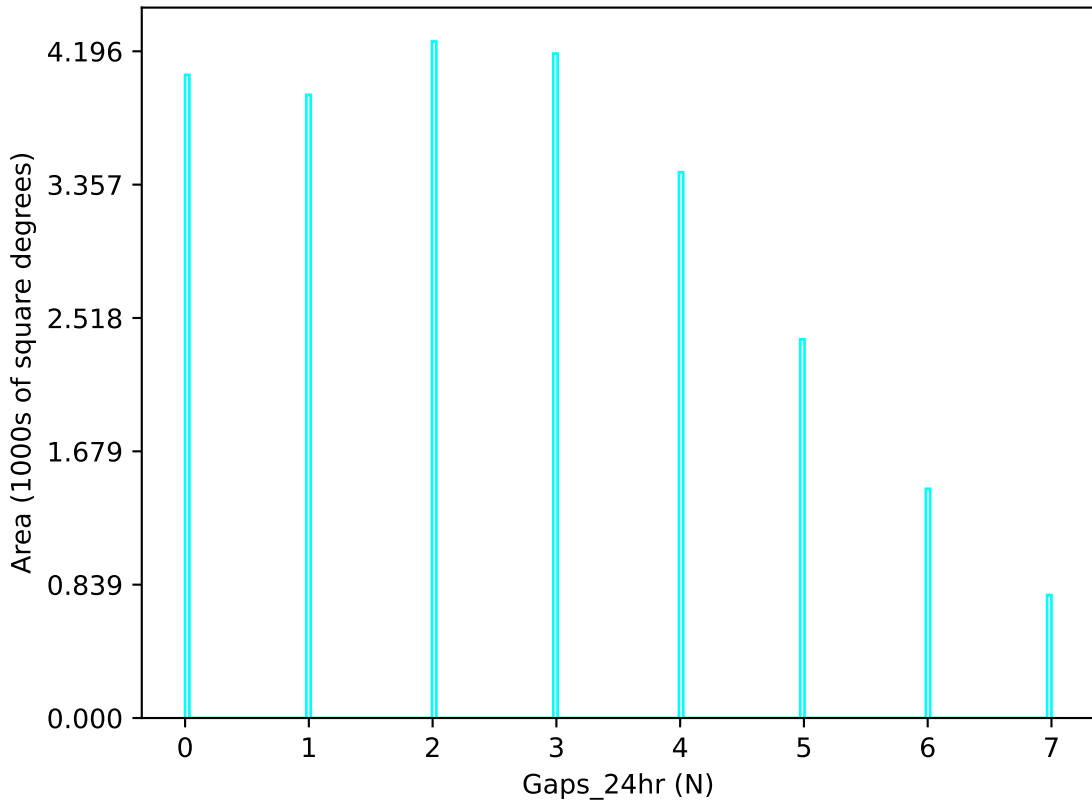
too_5_4v3.4_10yrs u band: Gaps_24hr
