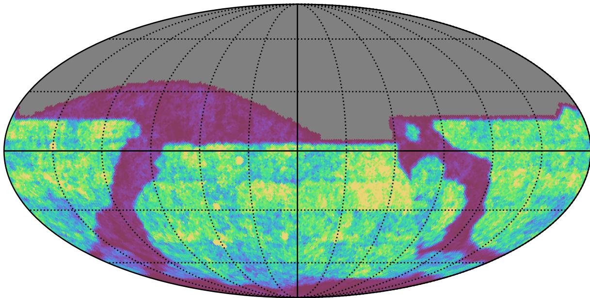
too_5_4v3.4_10yrs r band: Gaps_24hr
