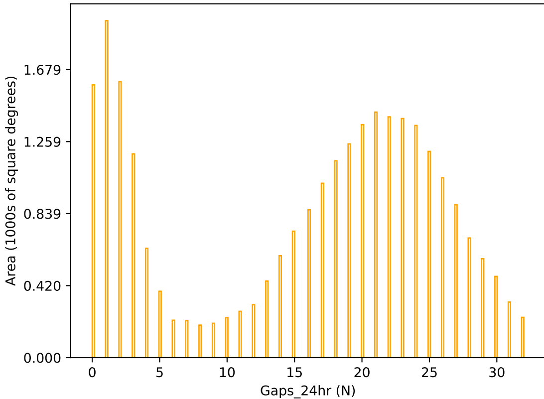
too_5_4v3.4_10yrs r band: Gaps_24hr
