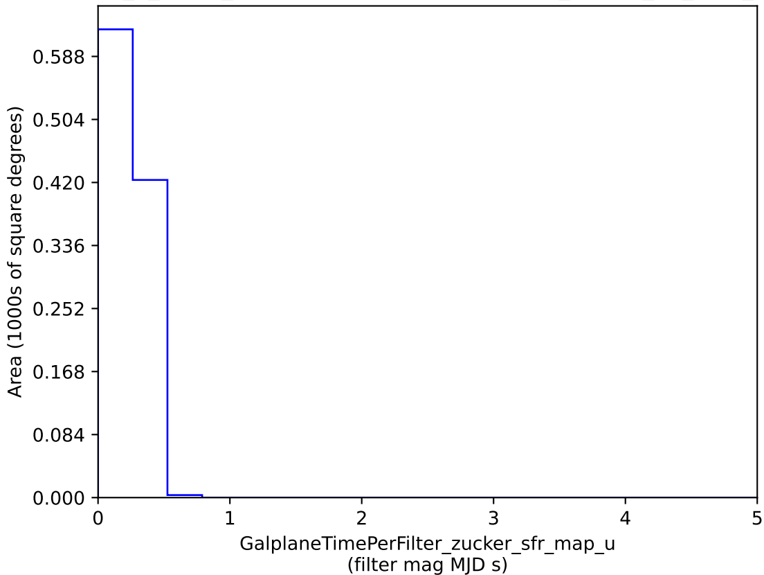
too_5_4v3.4_10yrs : GalplaneTimePerFilter_zucker_sfr_map_u
