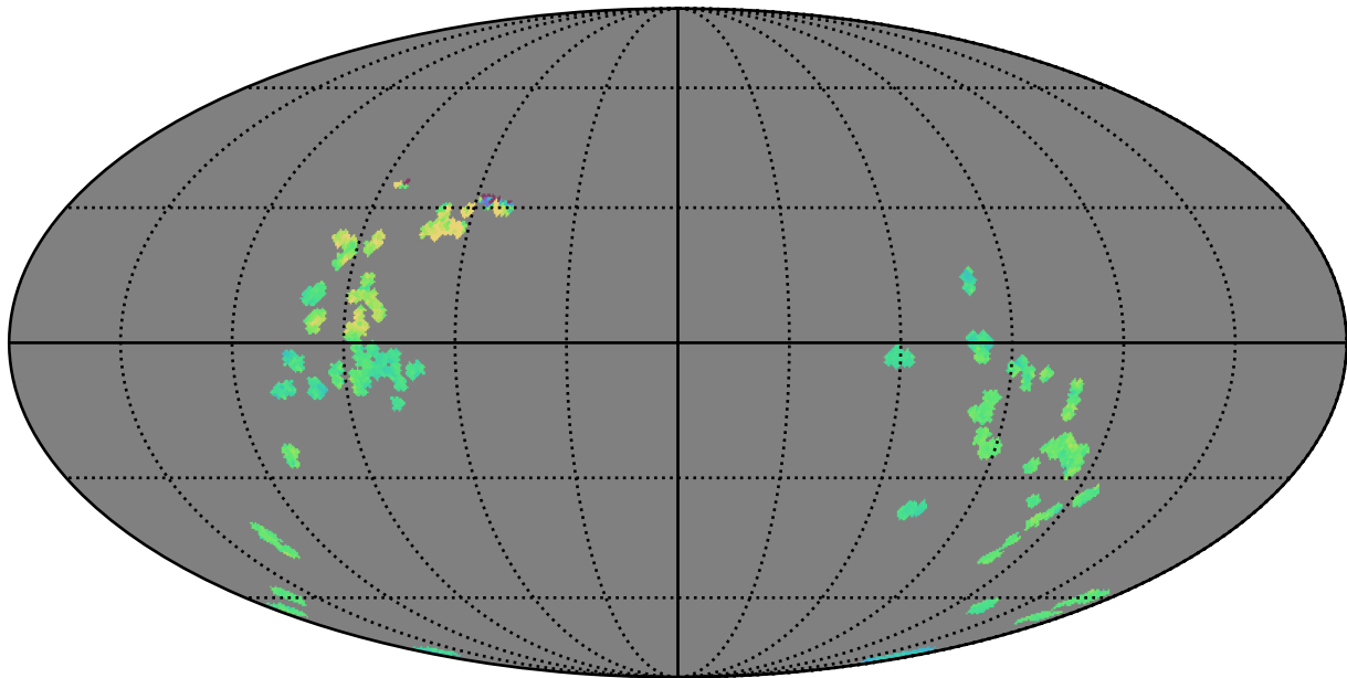
too_5_4v3.4_10yrs : GalplaneTimePerFilter_zucker_sfr_map_i
