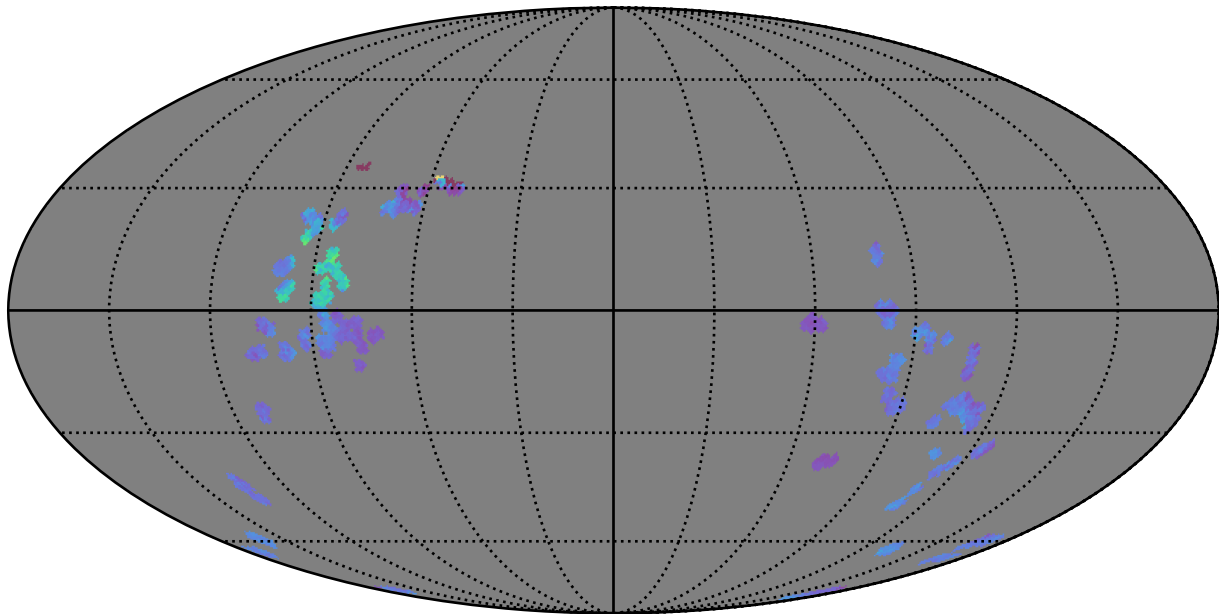
too_5_4v3.4_10yrs : GalplaneTimePerFilter_zucker_sfr_map_g
