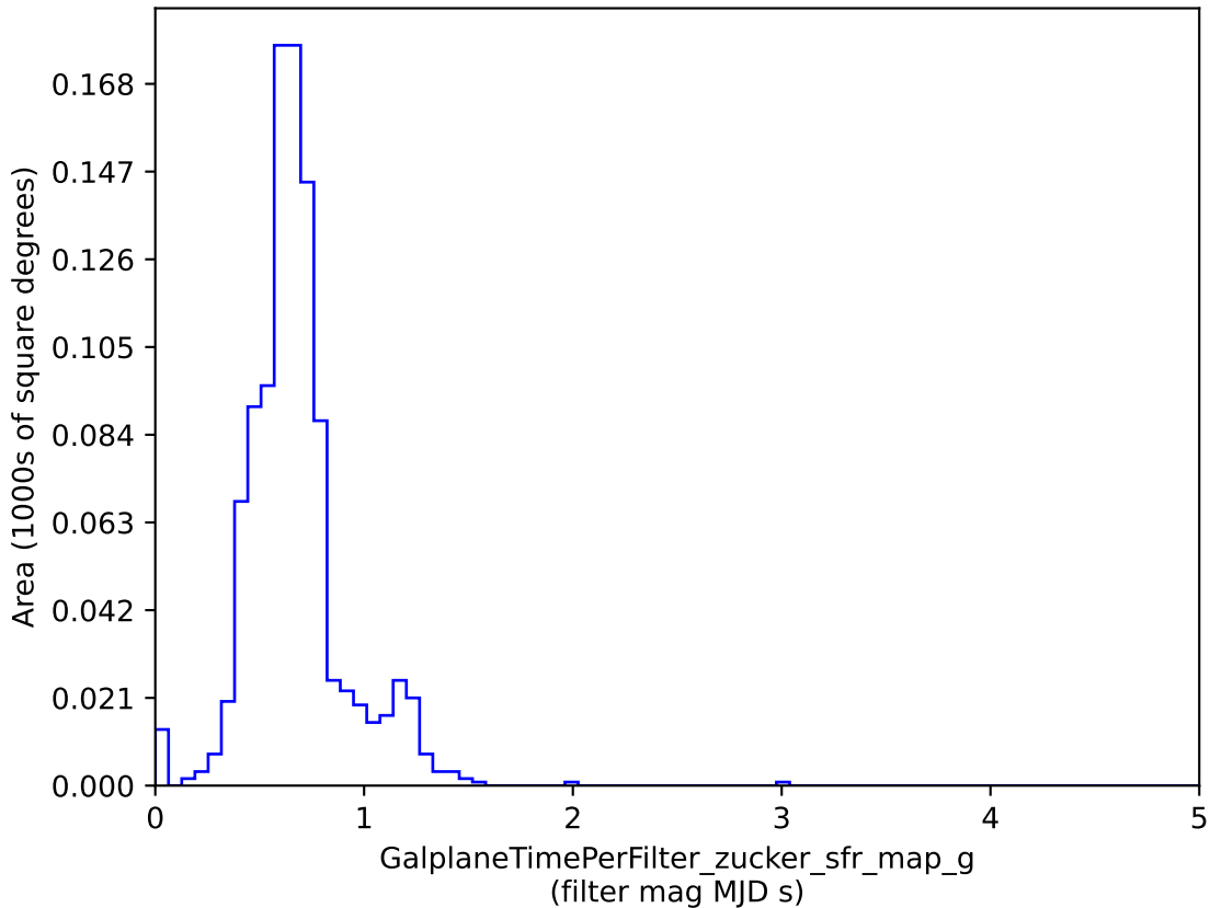
too_5_4v3.4_10yrs : GalplaneTimePerFilter_zucker_sfr_map_g
