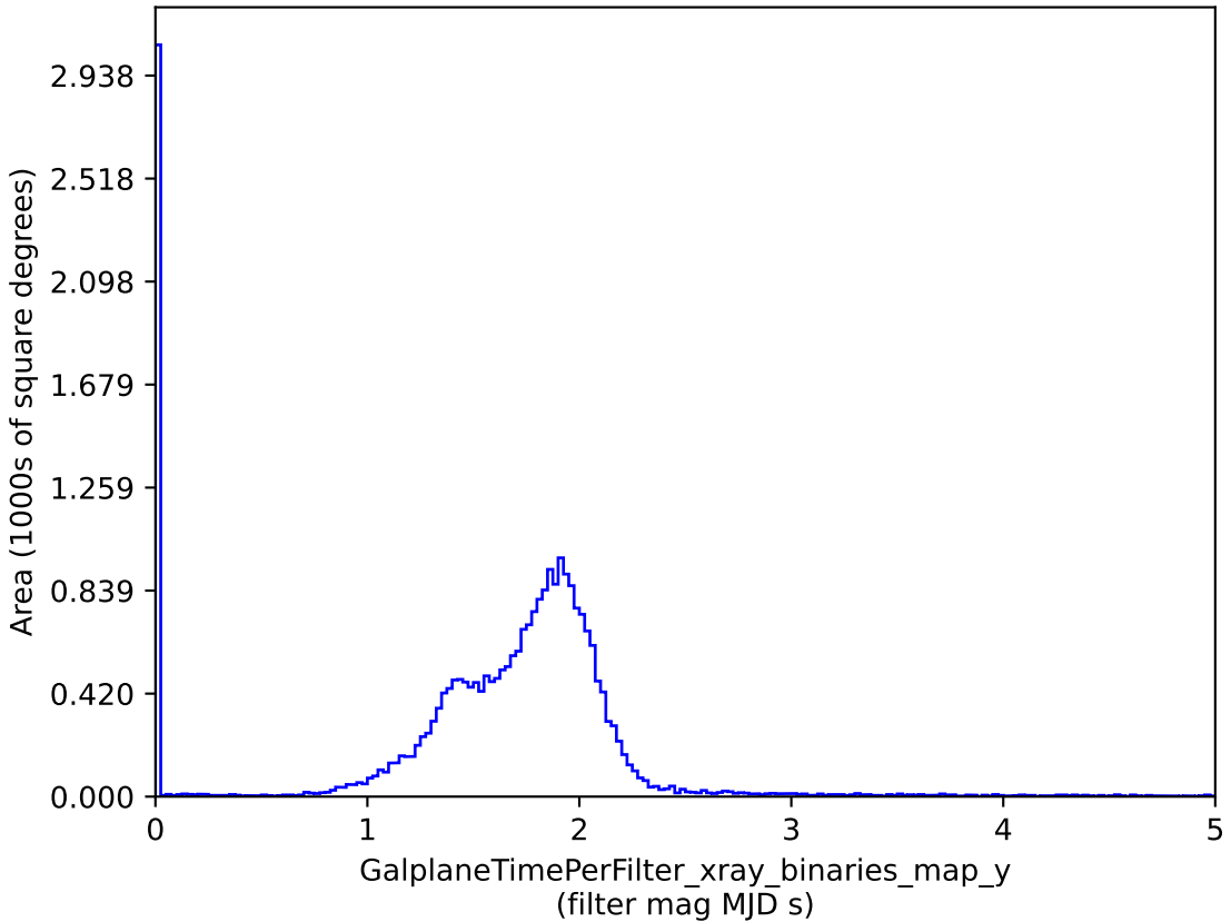
too_5_4v3.4_10yrs : GalplaneTimePerFilter_xray_binaries_map_y
