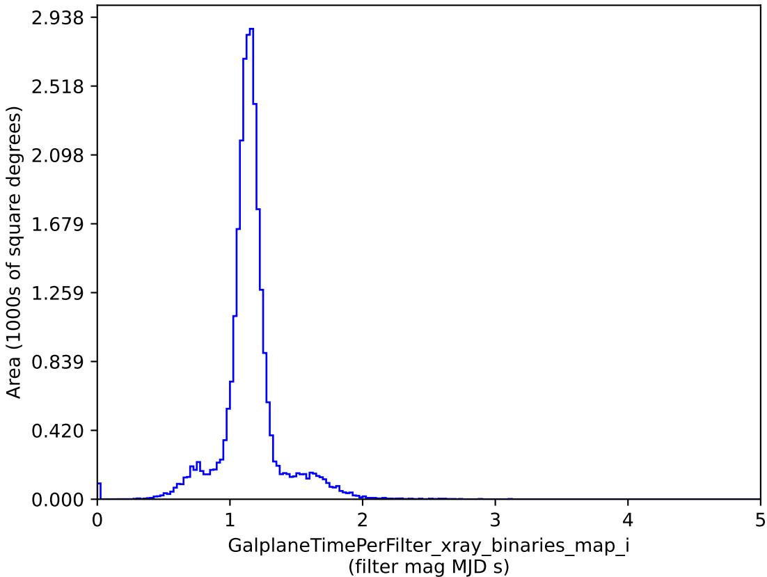
too_5_4v3.4_10yrs : GalplaneTimePerFilter_xray_binaries_map_i
