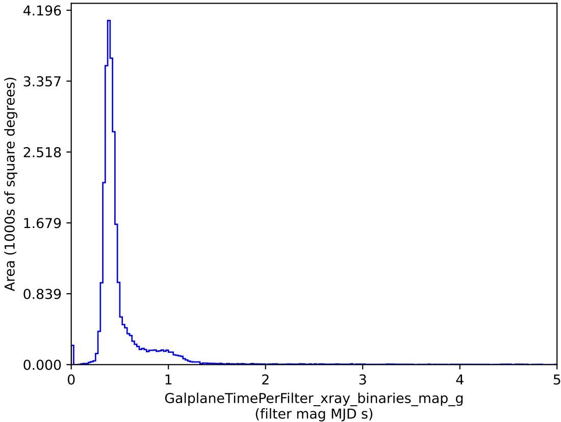
too_5_4v3.4_10yrs : GalplaneTimePerFilter_xray_binaries_map_g
