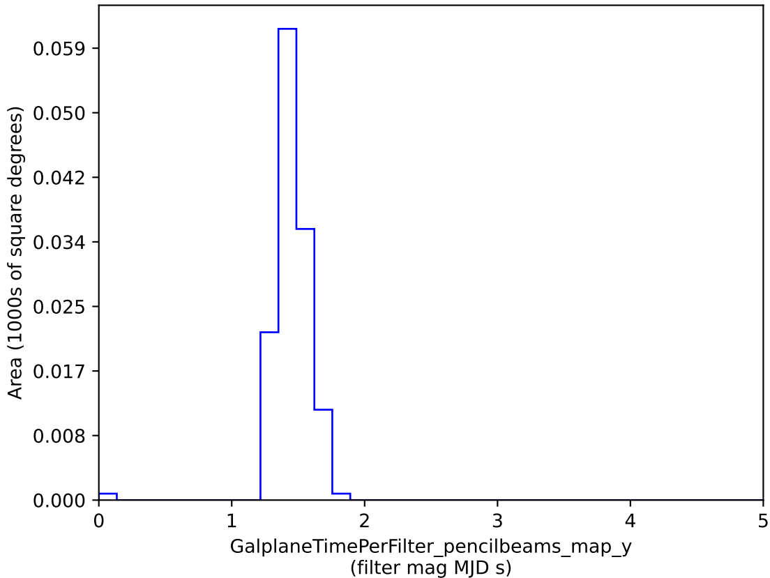
too_5_4v3.4_10yrs : GalplaneTimePerFilter_pencilbeams_map_y
