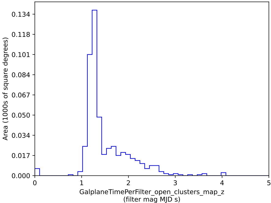
too_5_4v3.4_10yrs : GalplaneTimePerFilter_open_clusters_map_z
