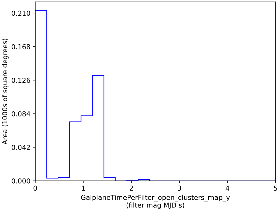
too_5_4v3.4_10yrs : GalplaneTimePerFilter_open_clusters_map_y
