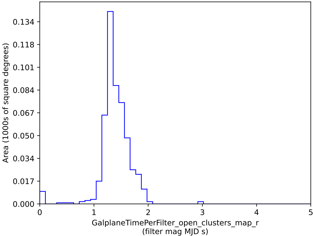
too_5_4v3.4_10yrs : GalplaneTimePerFilter_open_clusters_map_r
