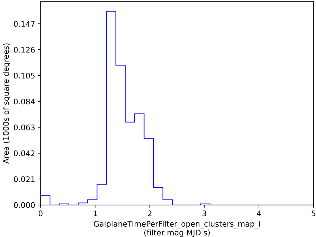
too_5_4v3.4_10yrs : GalplaneTimePerFilter_open_clusters_map_i
