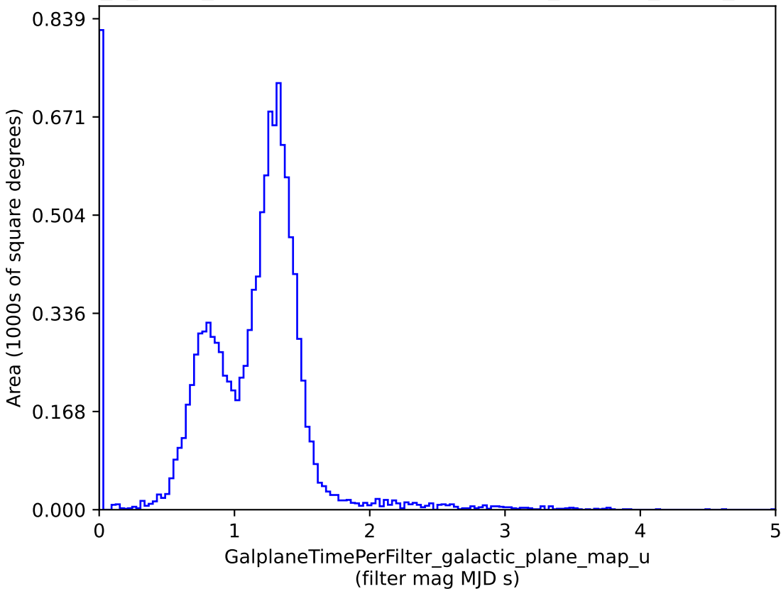
too_5_4v3.4_10yrs : GalplaneTimePerFilter_galactic_plane_map_u
