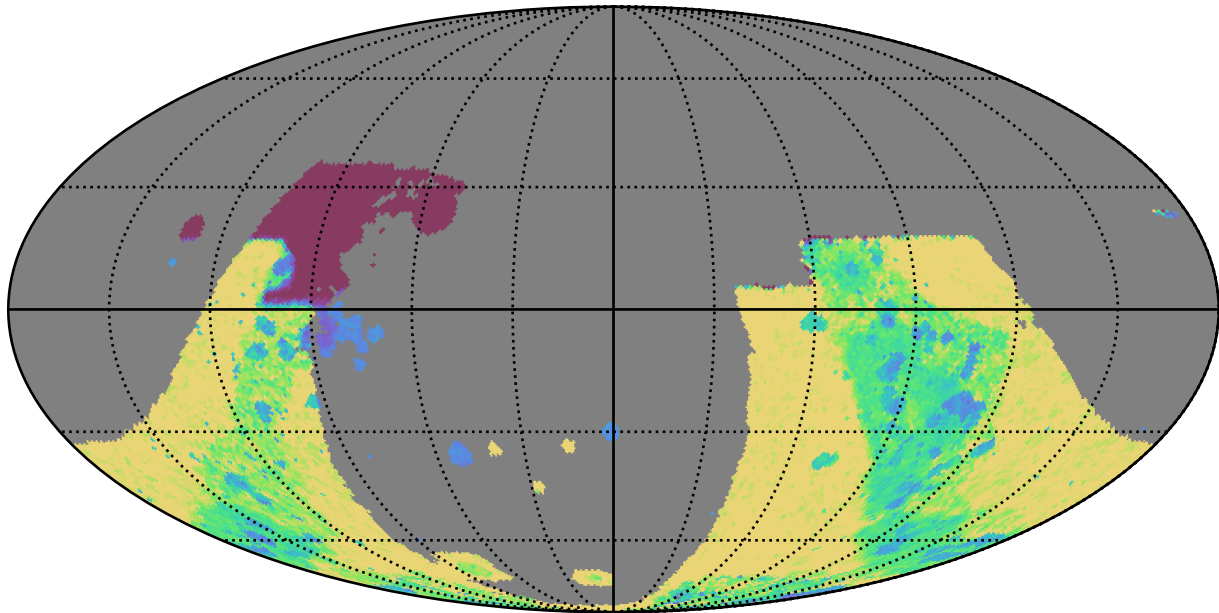
too_5_4v3.4_10yrs : GalplaneTimePerFilter_combined_map_y
