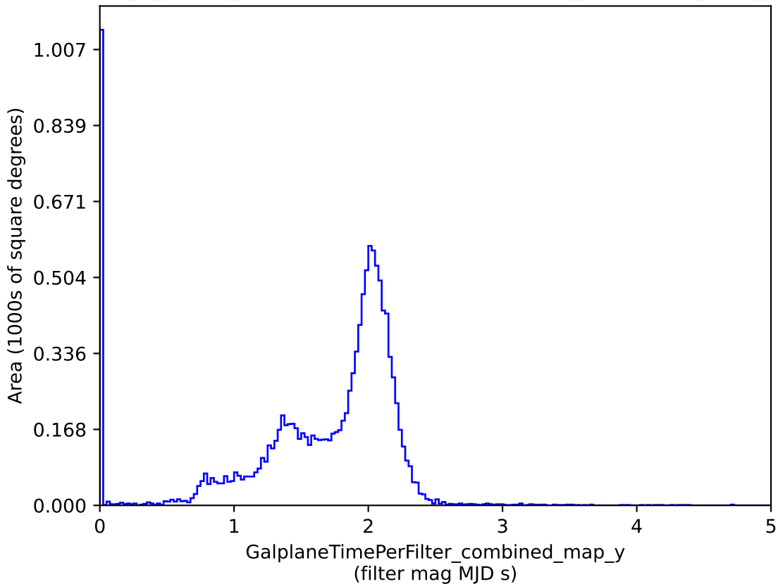
too_5_4v3.4_10yrs : GalplaneTimePerFilter_combined_map_y
