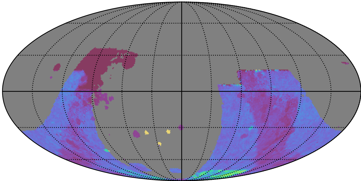
too_5_4v3.4_10yrs : GalplaneTimePerFilter_combined_map_u
