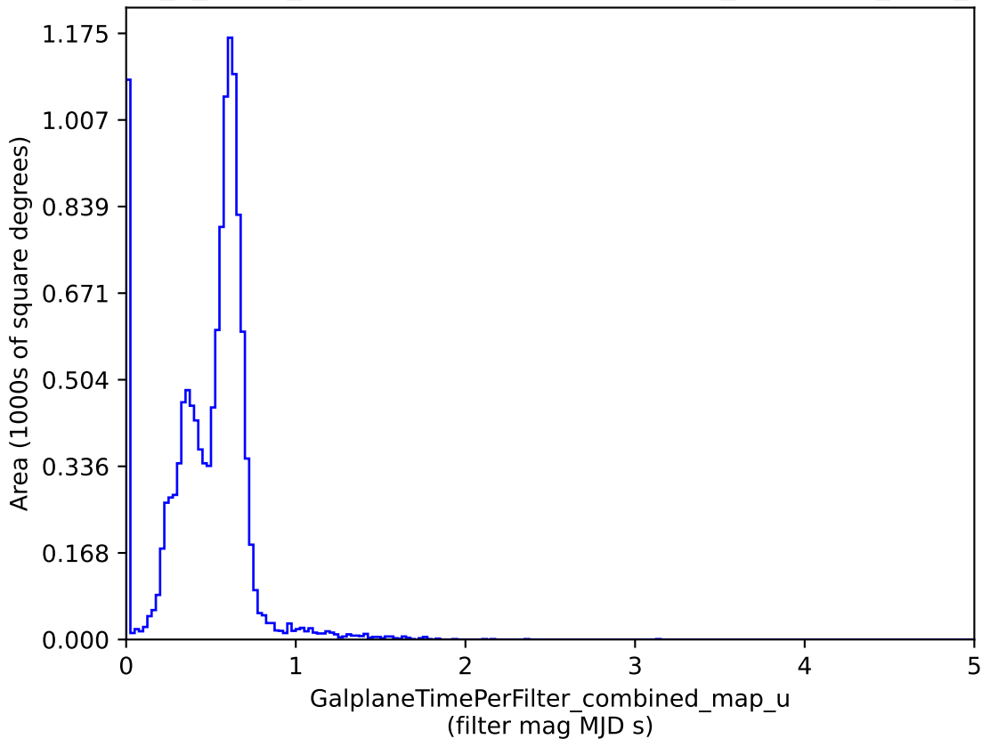
too_5_4v3.4_10yrs : GalplaneTimePerFilter_combined_map_u
