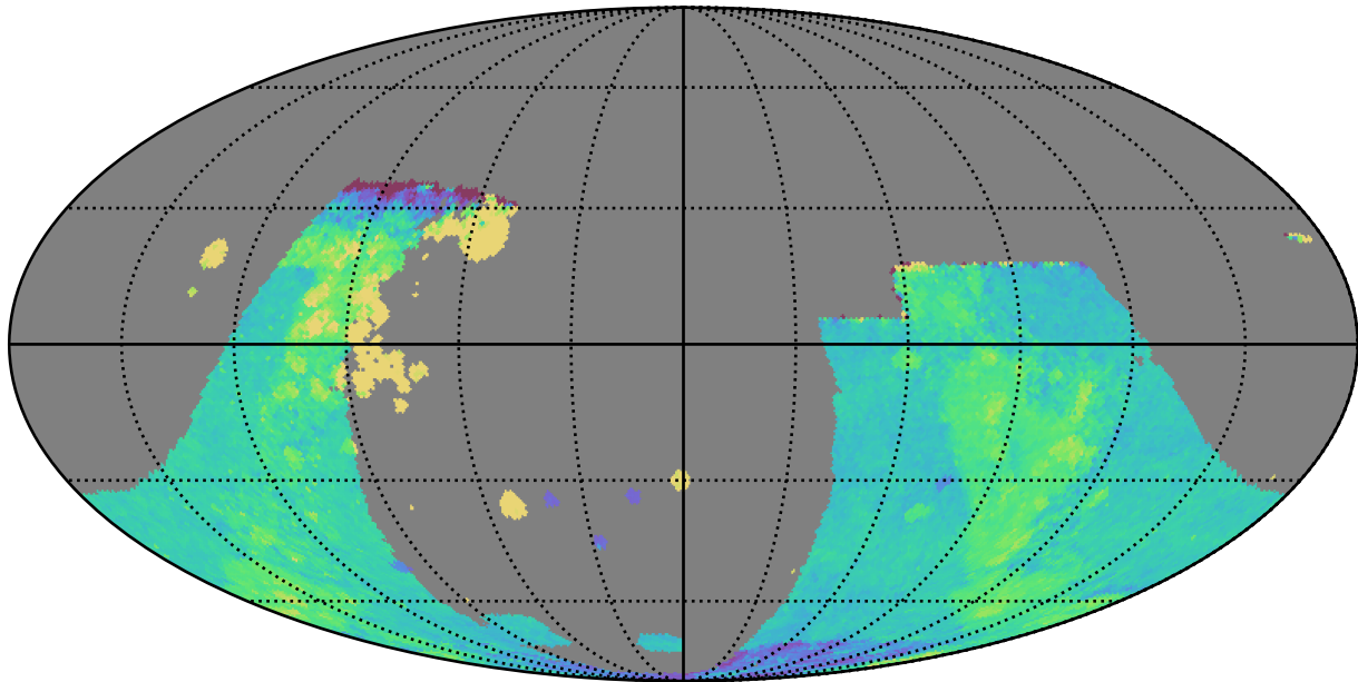
too_5_4v3.4_10yrs : GalplaneTimePerFilter_combined_map_r
