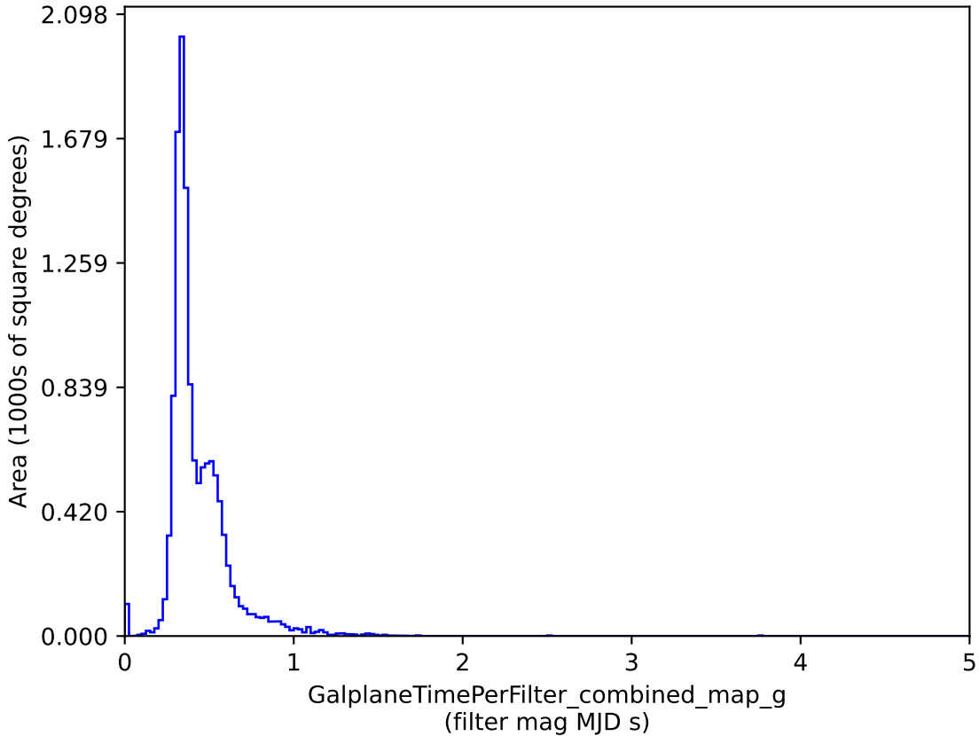
too_5_4v3.4_10yrs : GalplaneTimePerFilter_combined_map_g
