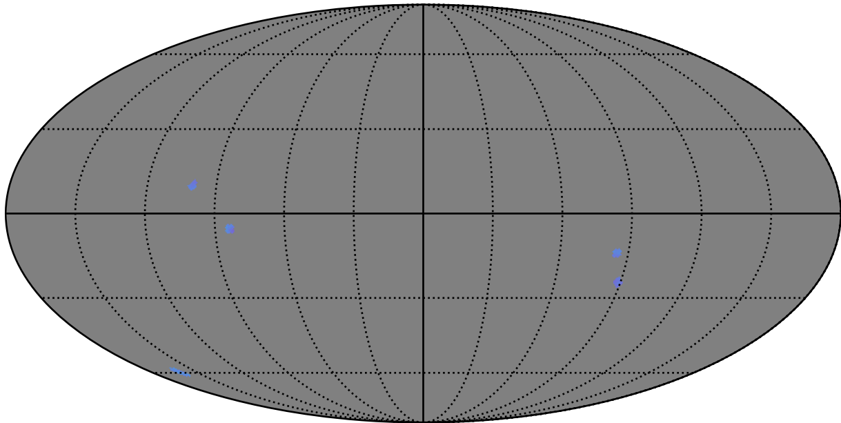
too_5_4v3.4_10yrs : GalplaneTimePerFilter_bonito_sfr_map_g
