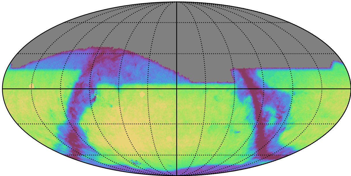
too_5_4v3.4_10yrs z: GalaxyCountsMetricExtended
