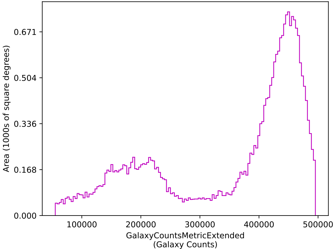
too_5_4v3.4_10yrs z: GalaxyCountsMetricExtended
