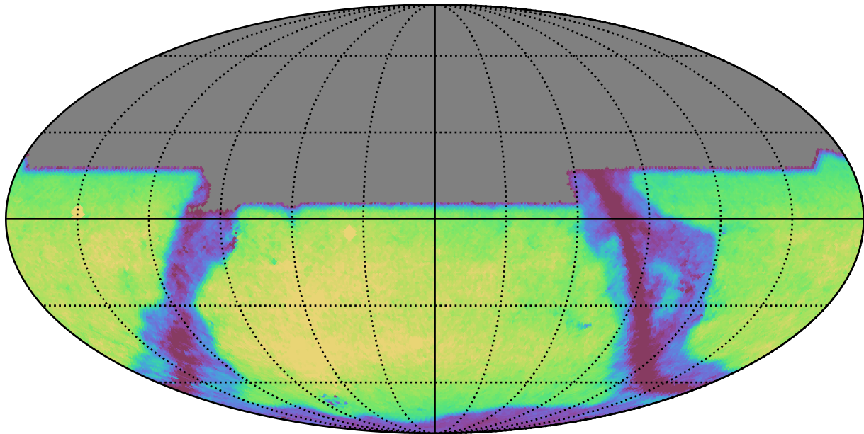
too_5_4v3.4_10yrs y: GalaxyCountsMetricExtended
