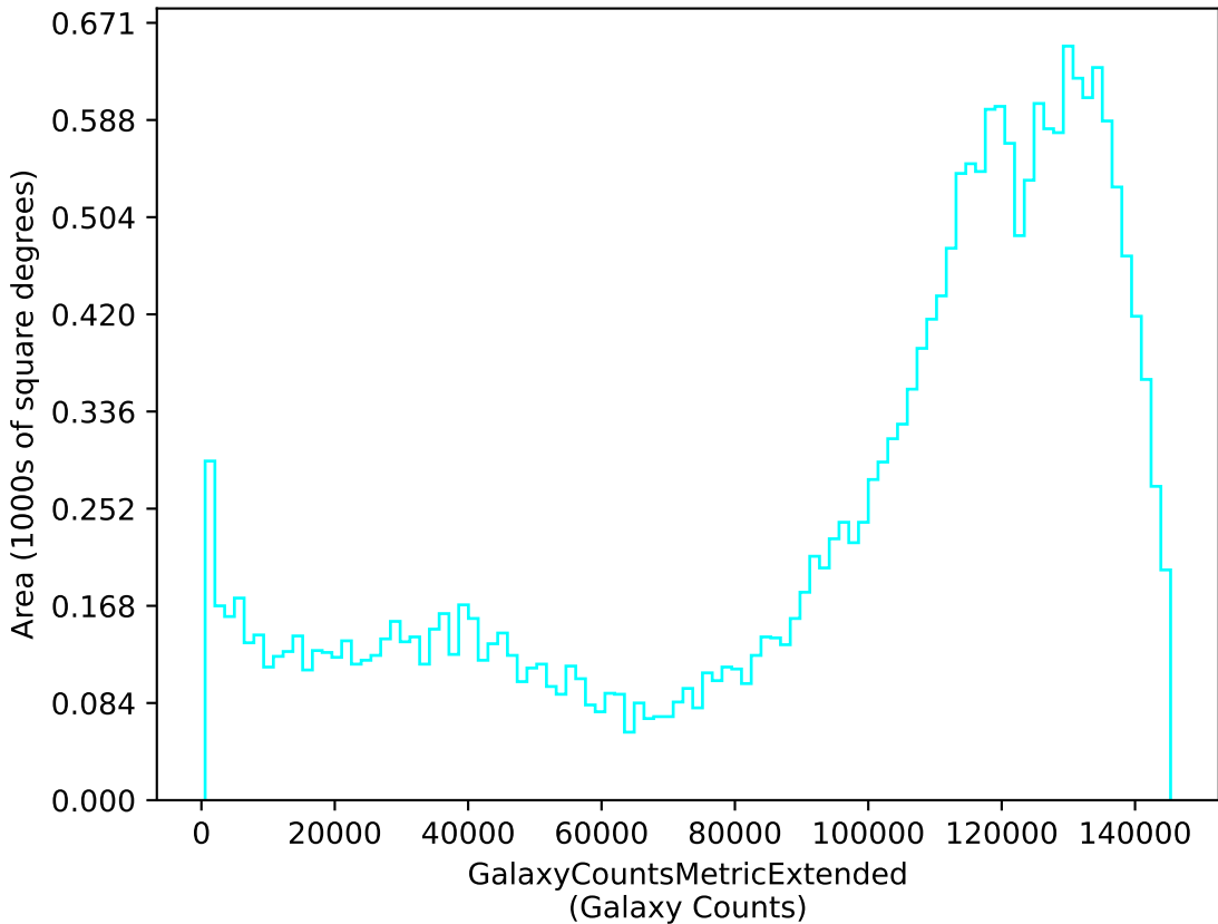
too_5_4v3.4_10yrs u: GalaxyCountsMetricExtended
