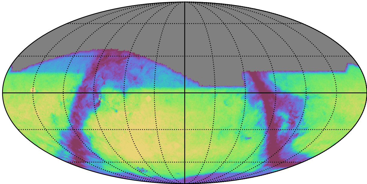
too_5_4v3.4_10yrs r: GalaxyCountsMetricExtended
