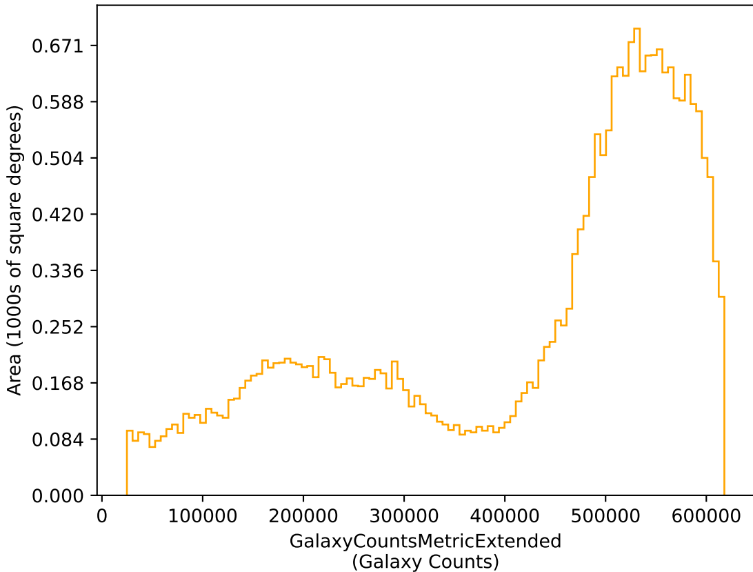
too_5_4v3.4_10yrs r: GalaxyCountsMetricExtended
