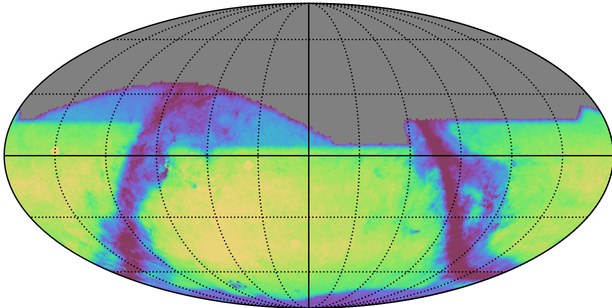
too_5_4v3.4_10yrs i: GalaxyCountsMetricExtended
