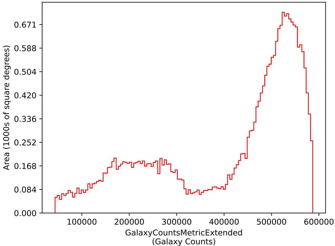
too_5_4v3.4_10yrs i: GalaxyCountsMetricExtended
